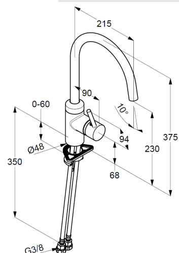
Dimensional drawing
